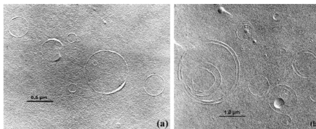
FIGURE 5. Freeze-fracture electron micrographs of cationic liposomes formed by (a) lipid 5a and (b) lipid 5a /DOPE (95:5 w/w).
