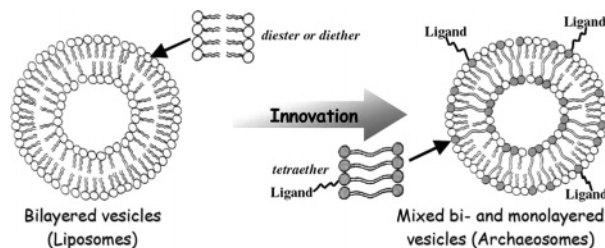
FIGURE 2. Stabilization of conventional liposome via the introduction of tetraether lipids.
