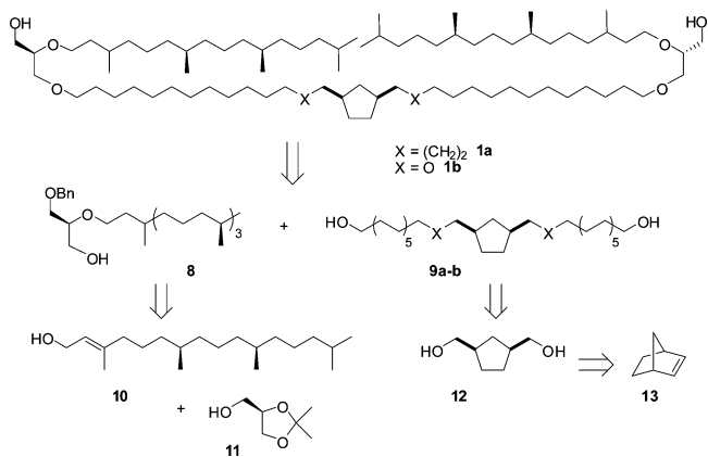
FIGURE 4. Retrosynthesis scheme tetraether analogues 1a,b .
