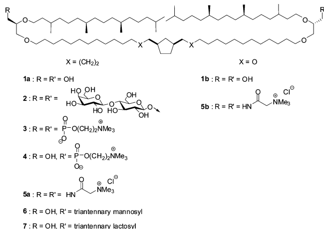
FIGURE 3. Synthetic analogues of archaeal membrane bipolar lipids.
