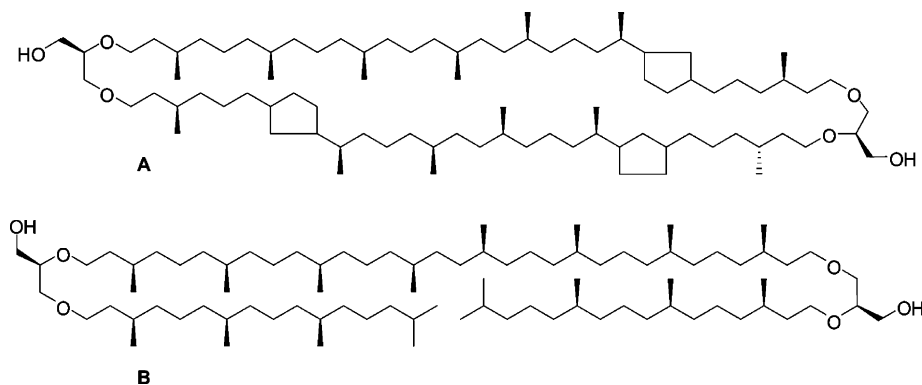
FIGURE 1. Typical basic structures of macrocyclic and hemimacrocyclic natural archaeal lipids.
